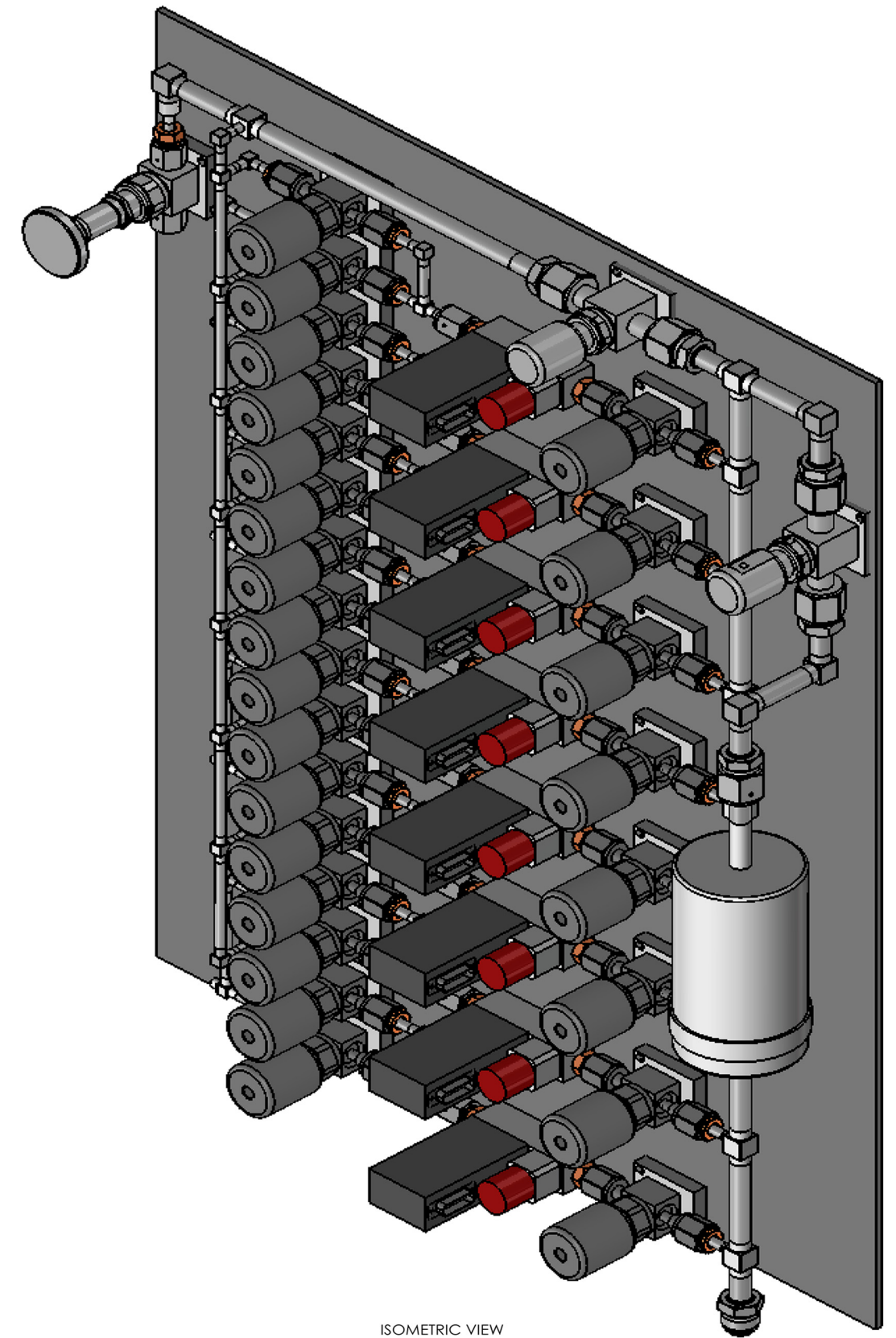
ISOMETRIC VIEW
